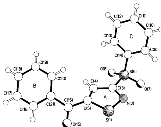
Fig. 3 The molecular structure of 8g .
