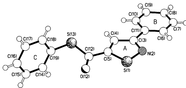
Fig. 5 The molecular structure of 13 .
