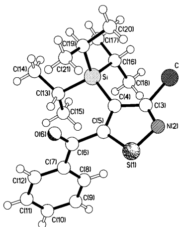
Fig. 8 The molecular structure of 9j .
