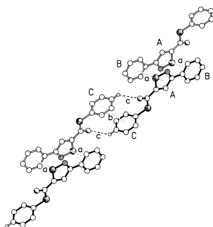
Fig. 6 Part of one of the continuous chains of molecules in the structure of 13 . The mean interplanar and centroid...centroid separations are (a) 3.60, 3.93 Å and (b) 3.58, 3.98 Å respectively. The C-H...O hydrogen bond (c) has C...O, H...O distances 3.30, 2.56 Å, and C-H...O angle 135°.
