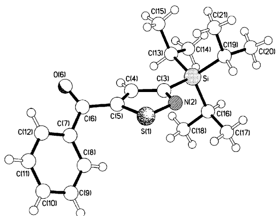
Fig. 7 The molecular structure of 8j .
