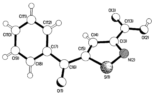
Fig. 1 The molecular structure of 8a .
