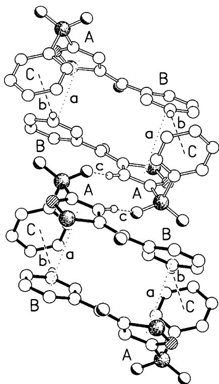
Fig. 4 Part of one of the continuous chains of linked "dimers" present in the structure of 8g . The respective mean interplanar and ring centroid...ring centroid separations are (a) 3.68, 3.91 Å. The C-H... \pi interaction (b) has H... \pi 2.82 Å and C-H... \pi 147°. The C-H...O hydrogen bond (c) has C...O, H...O distances 3.31, 2.40 Å, and C-H...O angle 157°.
