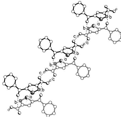
Fig. 2 Part of one of the continuous chains of molecules present in the structure of 8a . The respective mean interplanar and ring centroid \cdots ring centroid separations are ( a ) 3.59, 3.84 Å. The O \cdots C separation ( b ) is 3.15 Å. The O–H \cdots O hydrogen bond ( c ) has O \cdots O, H \cdots O distances 2.65, 1.75 Å, and O–H \cdots O angle 175°.
